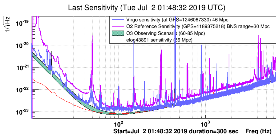
Figure 12 Virgo Sensitivity curve
