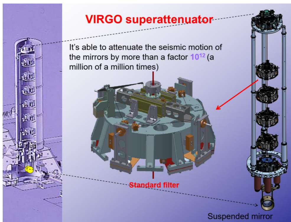
Figure 9 Virgo impressive seismic isolator: the superattenuator
