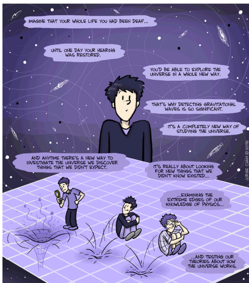
Figure 3 Astronomy status after gravitational wave detection.
