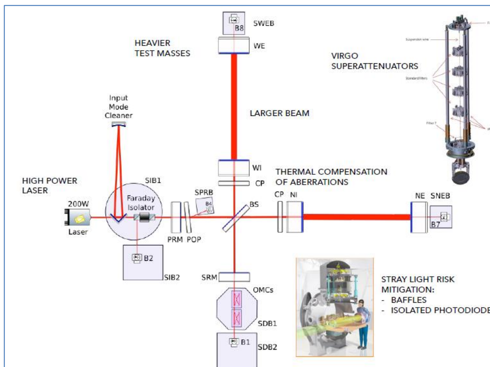
Figure 10 Optical scheme of Advanced Virgo, a modern GW detector
